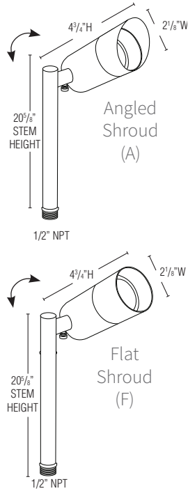
·FLAT SHROUD
