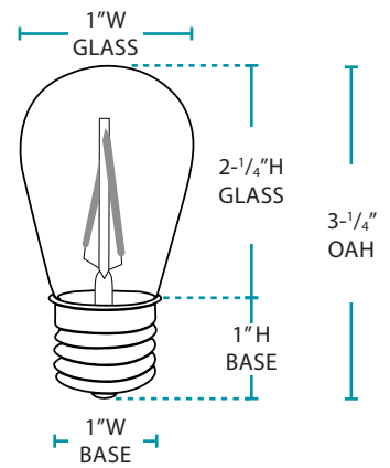
S14 LAMP DIMENSIONS
