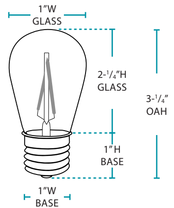
S14 LAMP DIMENSIONS
