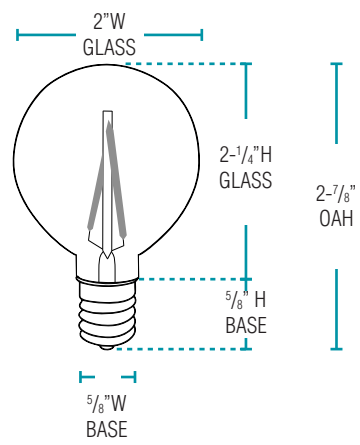
Dimensions for all G50 lamps on this page.
